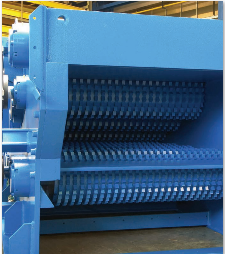
Unique infeed roller designs available, such as the above VTH 12-VU Paper Core Shredder, designed specifically for size reduction of paper cores.
